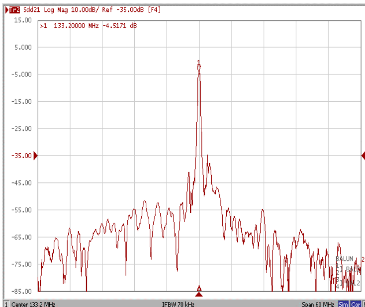
Frequency Response
