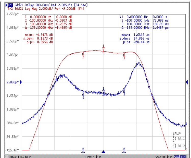
Ripple & Group Delay Variation Fo±100 KHz
